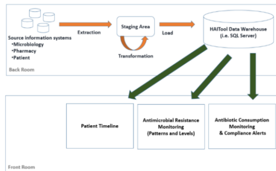
Figure 1. HAITool's architecture.
